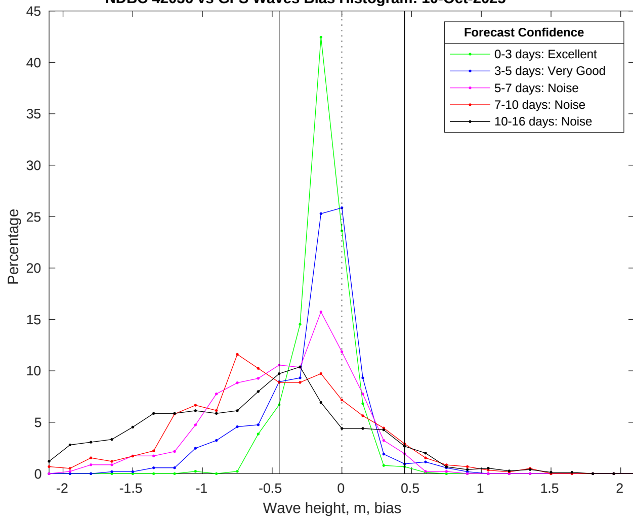
NDBC 42036 vs GFS Waves Bias Histogram: 10-Oct-2025
