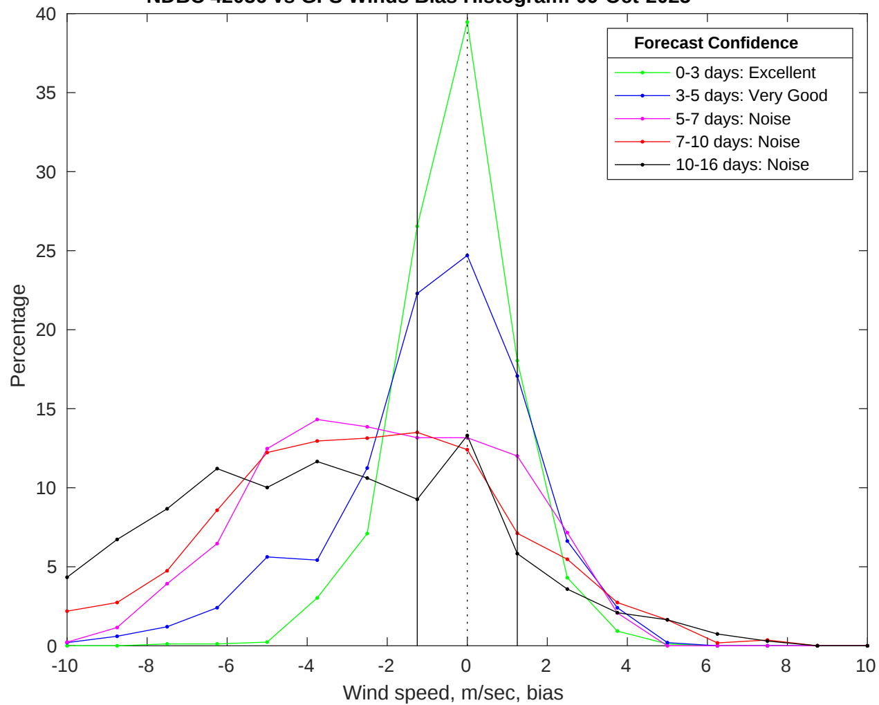
NDBC 42036 vs GFS Winds Bias Histogram: 09-Oct-2025
