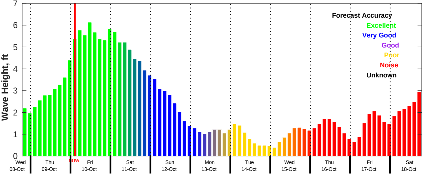
CMEMS Wave Forecast for NDBC 42036 from 08-Oct-2025 19:00:00 to 18-Oct-2025 19:00:00
