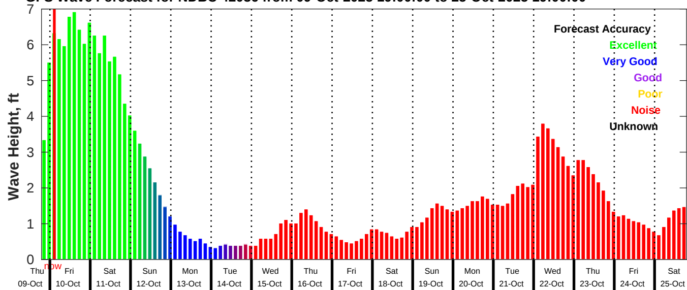
GFS Wave Forecast for NDBC 42036 from 09-Oct-2025 19:00:00 to 25-Oct-2025 19:00:00
