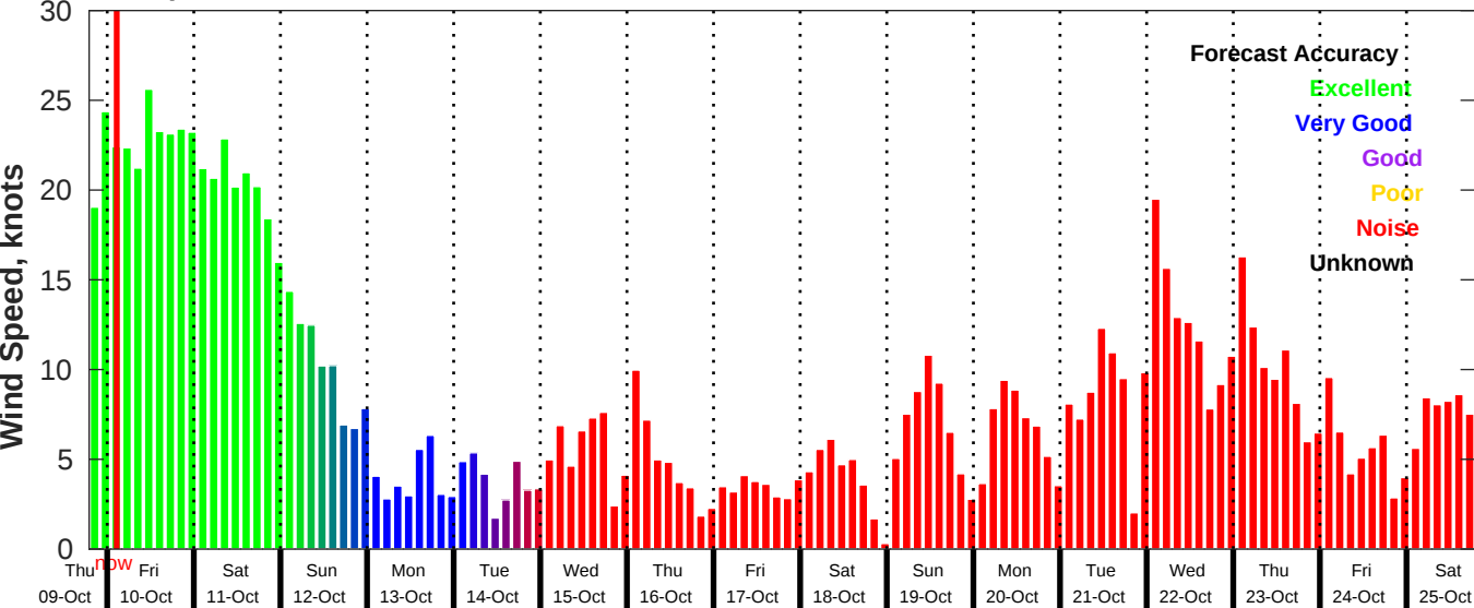
GFS Wind Speed Forecast for NDBC 42036 from 09-Oct-2025 19:00:00 to 25-Oct-2025 19:00:00
