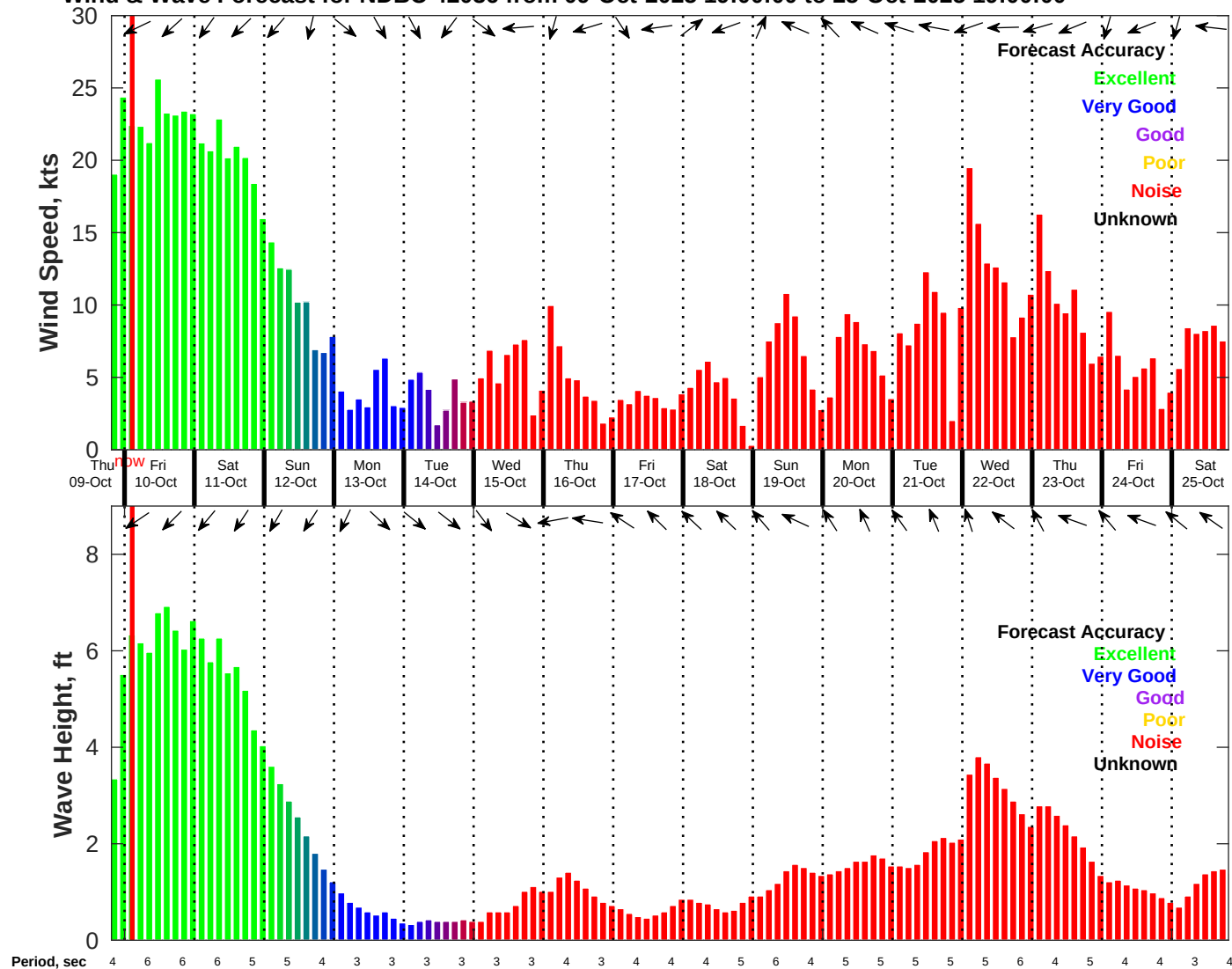
Wind & Wave Forecast for NDBC 42036 from 09-Oct-2025 19:00:00 to 25-Oct-2025 19:00:00
