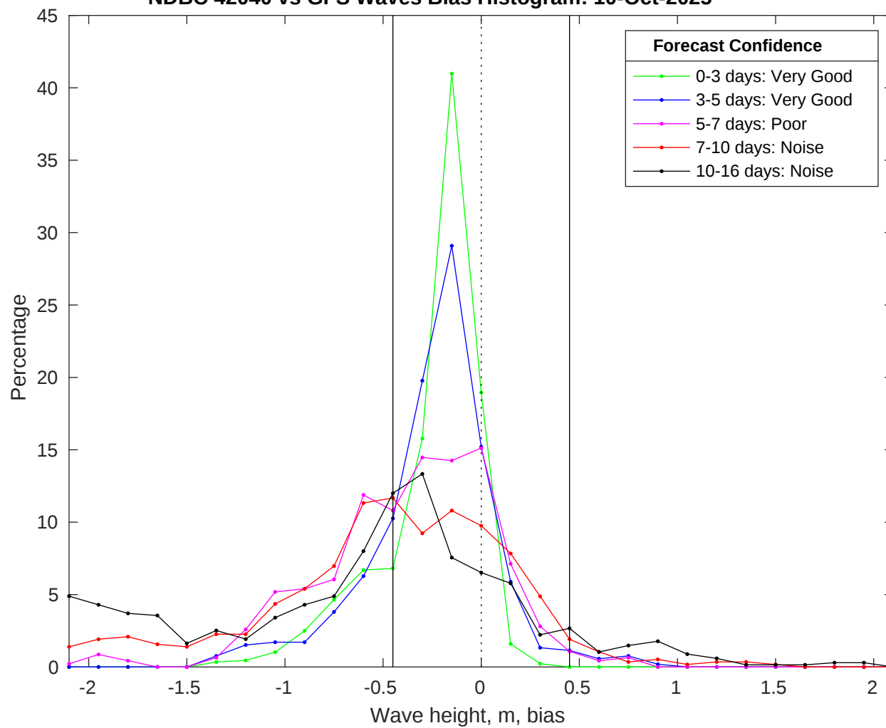
NDBC 42040 vs GFS Waves Bias Histogram: 10-Oct-2025
