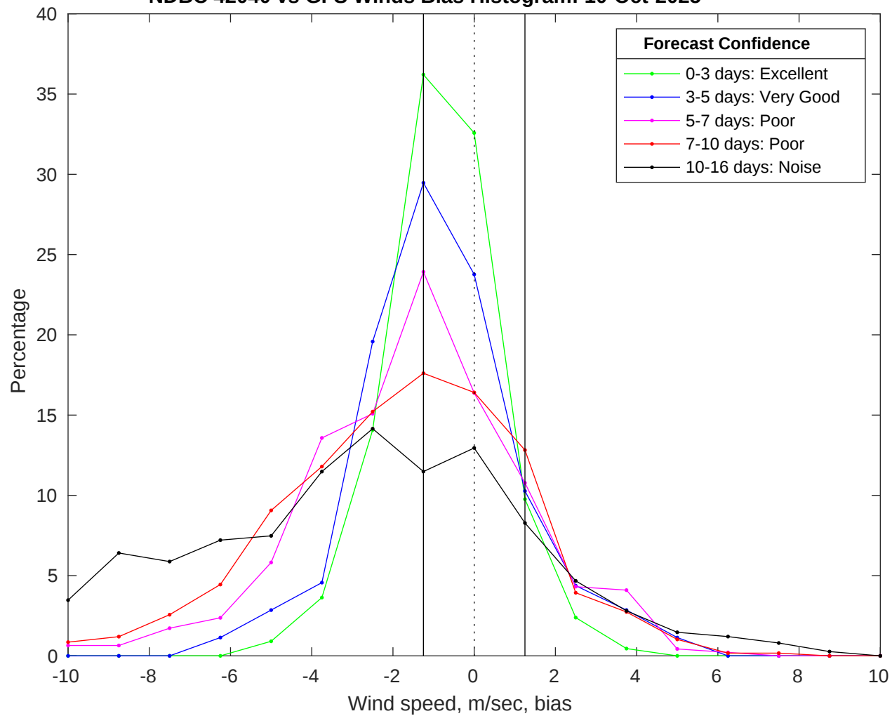
NDBC 42040 vs GFS Winds Bias Histogram: 10-Oct-2025
