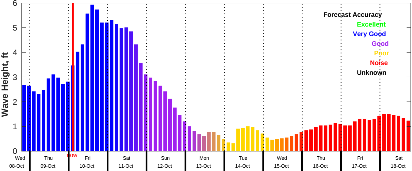
CMEMS Wave Forecast for NDBC 42040 from 08-Oct-2025 19:00:00 to 18-Oct-2025 19:00:00
