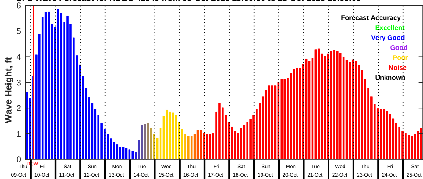
GFS Wave Forecast for NDBC 42040 from 09-Oct-2025 19:00:00 to 25-Oct-2025 19:00:00
