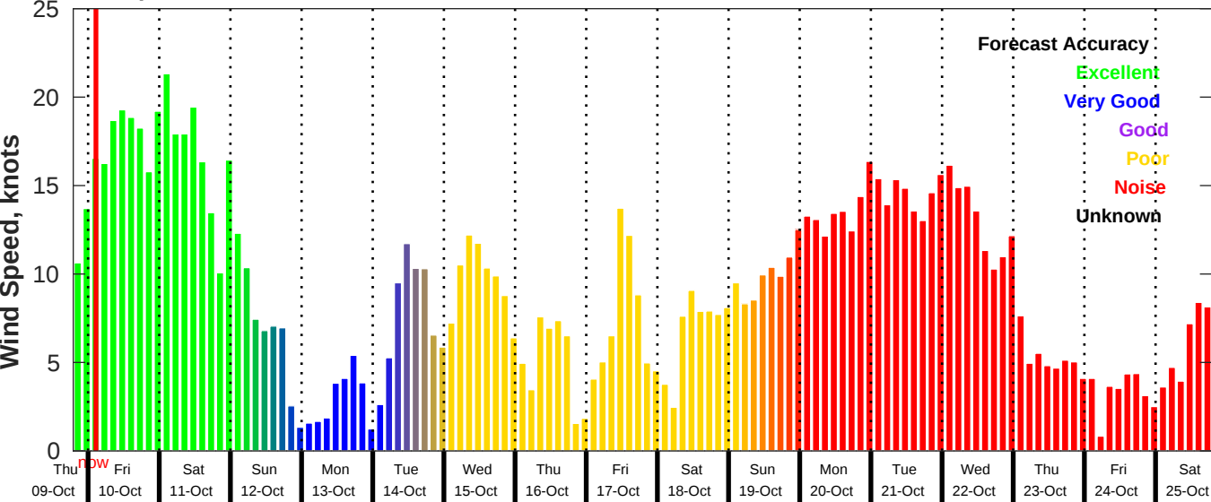
GFS Wind Speed Forecast for NDBC 42040 from 09-Oct-2025 19:00:00 to 25-Oct-2025 19:00:00
