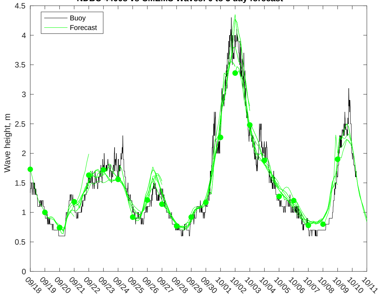
NDBC 44008 vs CMEMS Waves: 0 to 3 day forecast
