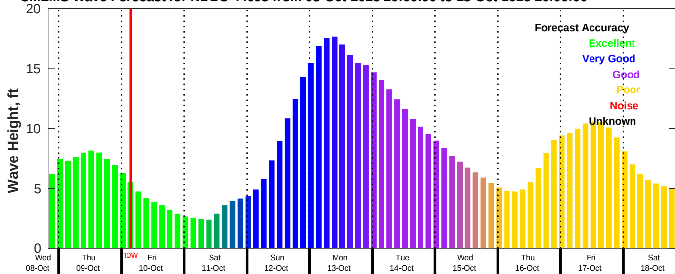
CMEMS Wave Forecast for NDBC 44008 from 08-Oct-2025 20:00:00 to 18-Oct-2025 20:00:00
