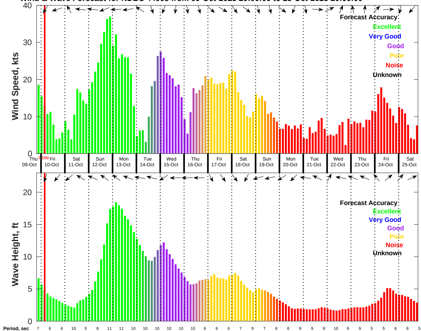
Wind & Wave Forecast for NDBC 44008 from 09-Oct-2025 20:00:00 to 25-Oct-2025 20:00:00
