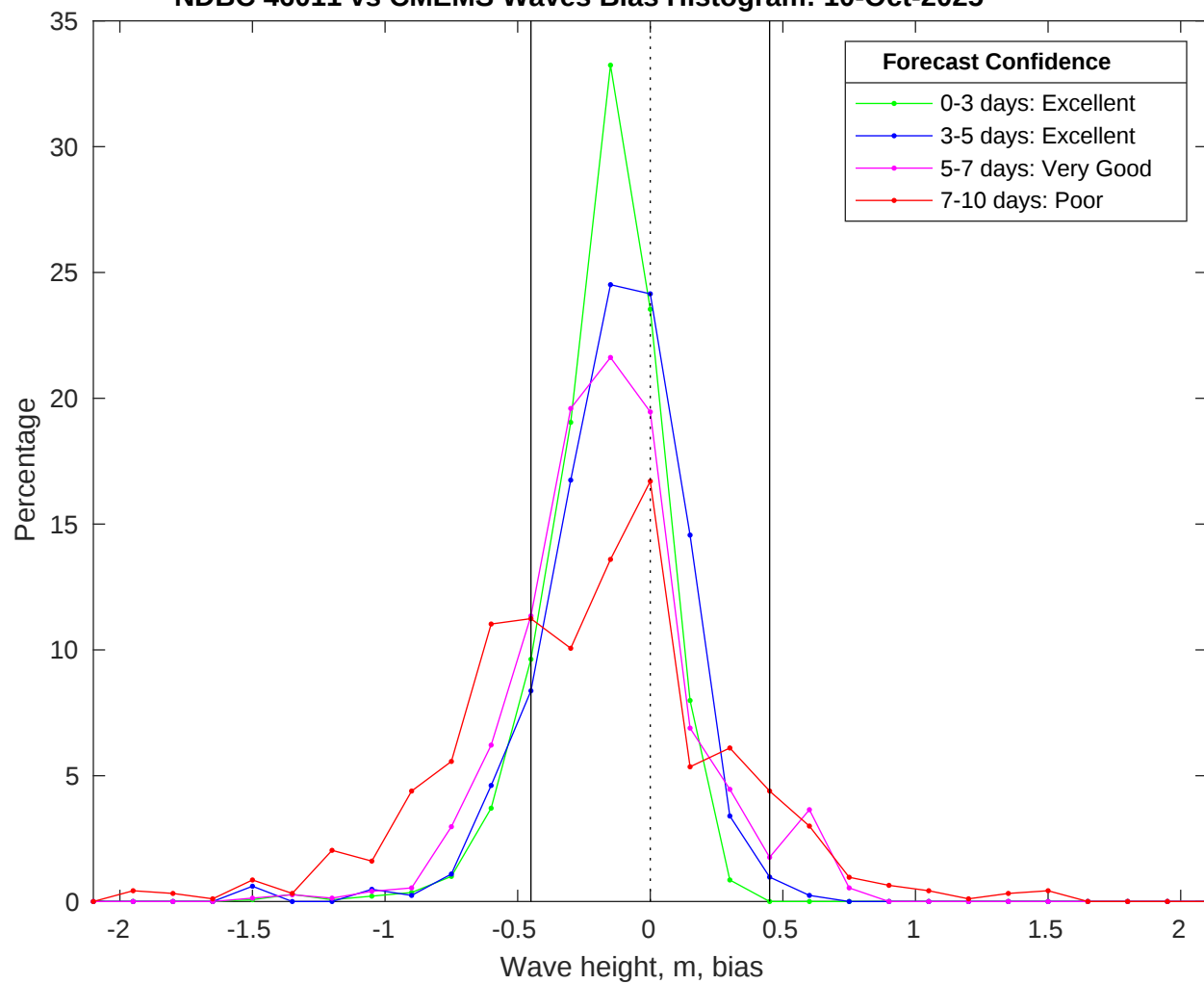
NDBC 46011 vs CMEMS Waves Bias Histogram: 10-Oct-2025
