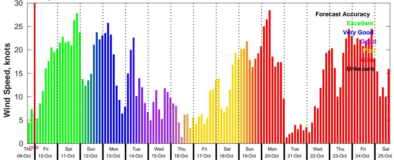
GFS Wind Speed Forecast for NDBC 46011 from 09-Oct-2025 16:00:00 to 25-Oct-2025 16:00:00
