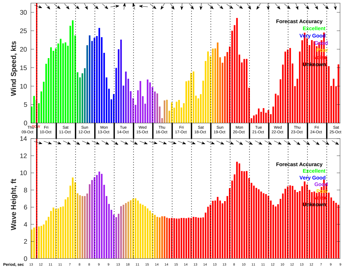
Wind & Wave Forecast for NDBC 46011 from 09-Oct-2025 16:00:00 to 25-Oct-2025 16:00:00
