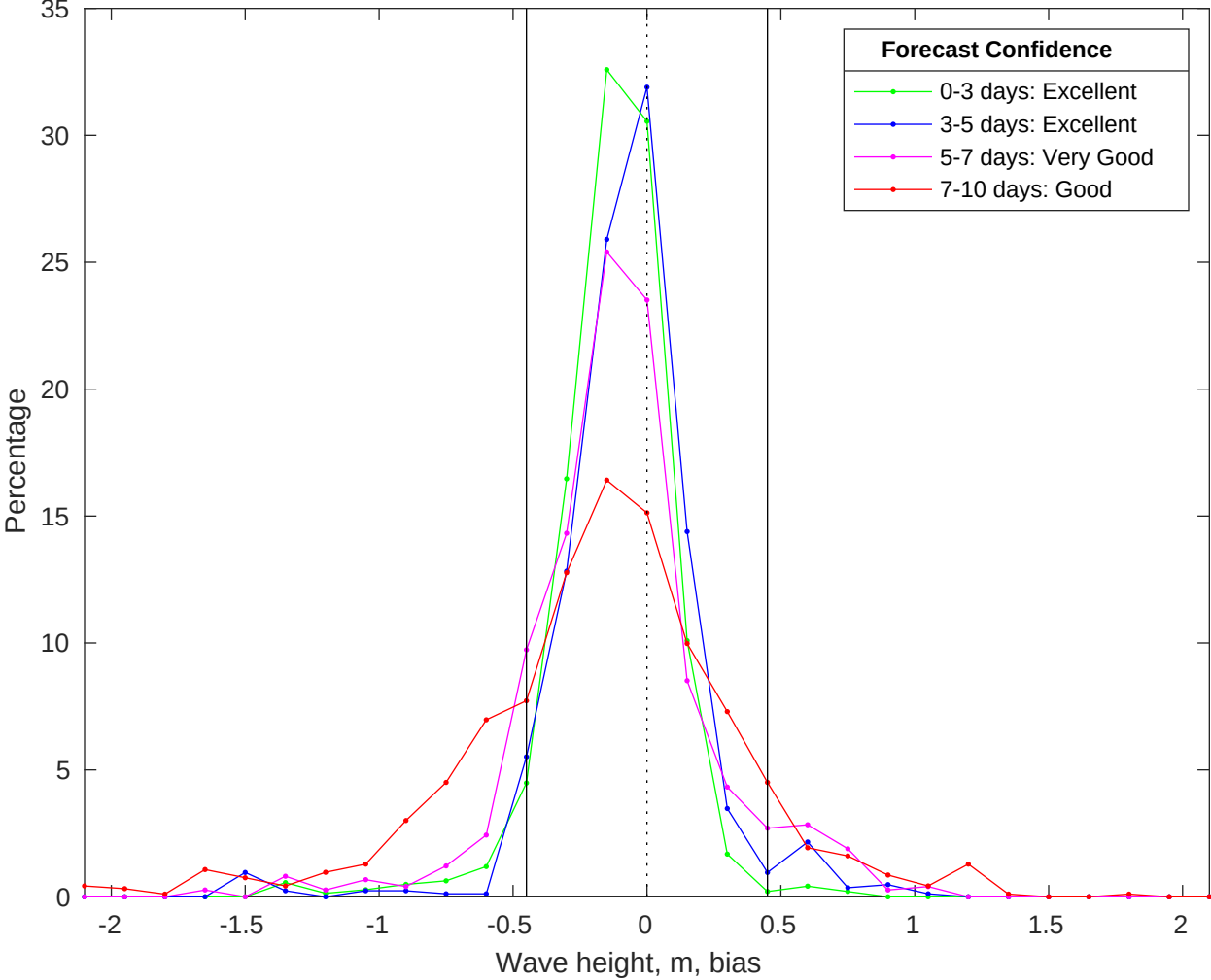
NDBC 46028 vs CMEMS Waves Bias Histogram: 10-Oct-2025
