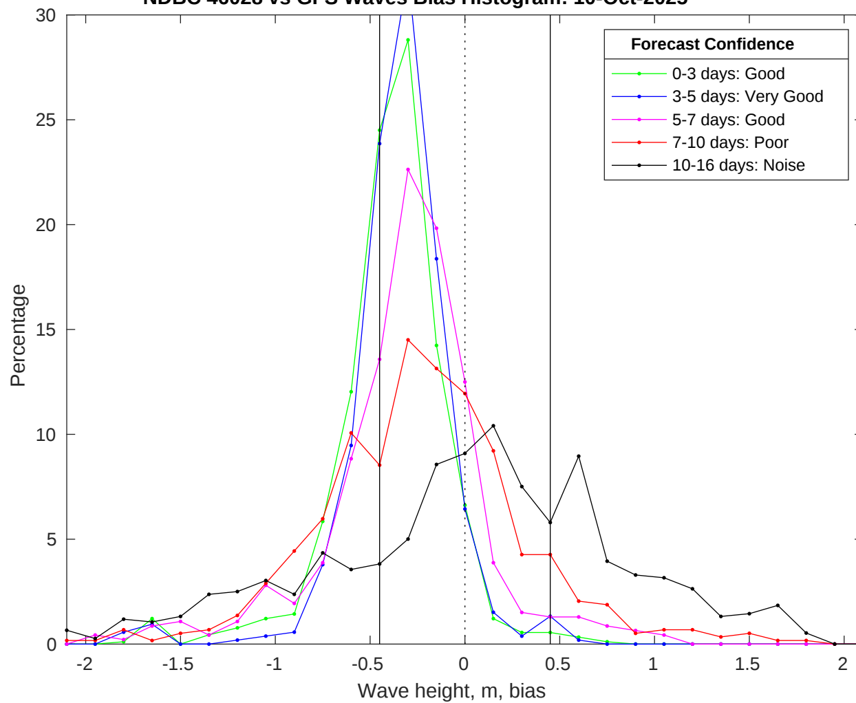
NDBC 46028 vs GFS Waves Bias Histogram: 10-Oct-2025
