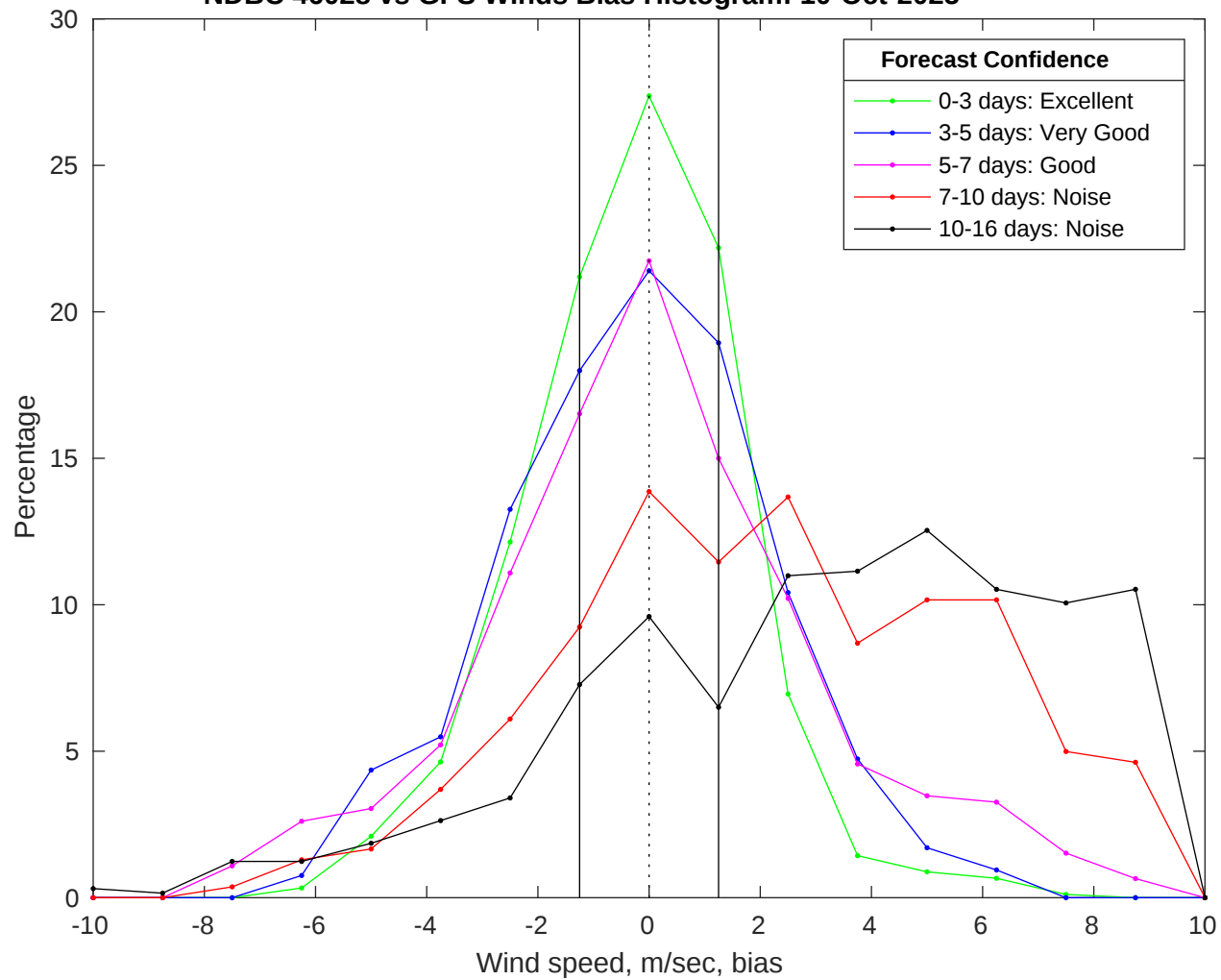
NDBC 46028 vs GFS Winds Bias Histogram: 10-Oct-2025
