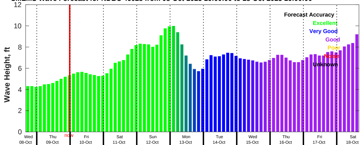
CMEMS Wave Forecast for NDBC 46028 from 08-Oct-2025 16:00:00 to 18-Oct-2025 16:00:00
