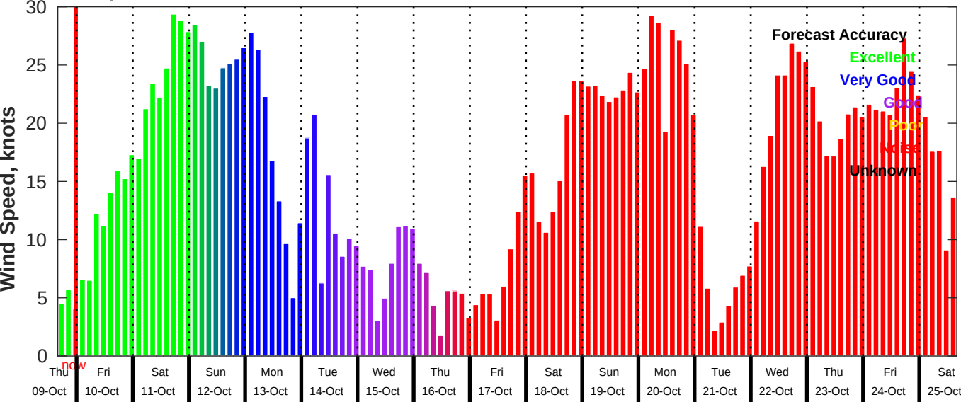
GFS Wind Speed Forecast for NDBC 46028 from 09-Oct-2025 16:00:00 to 25-Oct-2025 16:00:00
