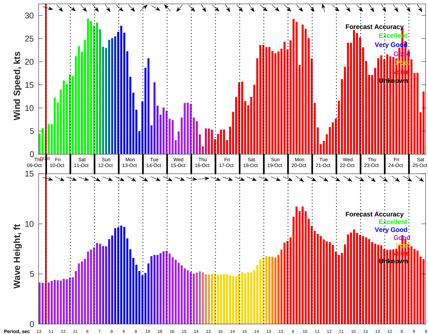
Wind & Wave Forecast for NDBC 46028 from 09-Oct-2025 16:00:00 to 25-Oct-2025 16:00:00
