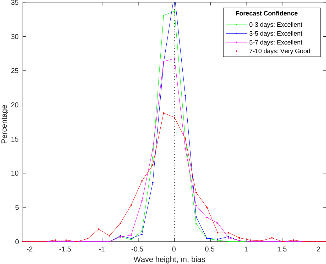
NDBC 46054 vs CMEMS Waves Bias Histogram: 10-Oct-2025
