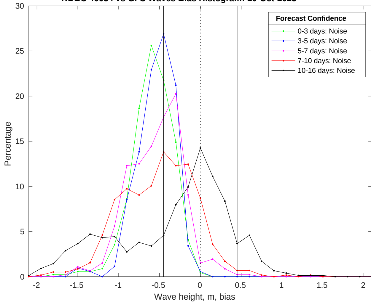
NDBC 46054 vs GFS Waves Bias Histogram: 10-Oct-2025
