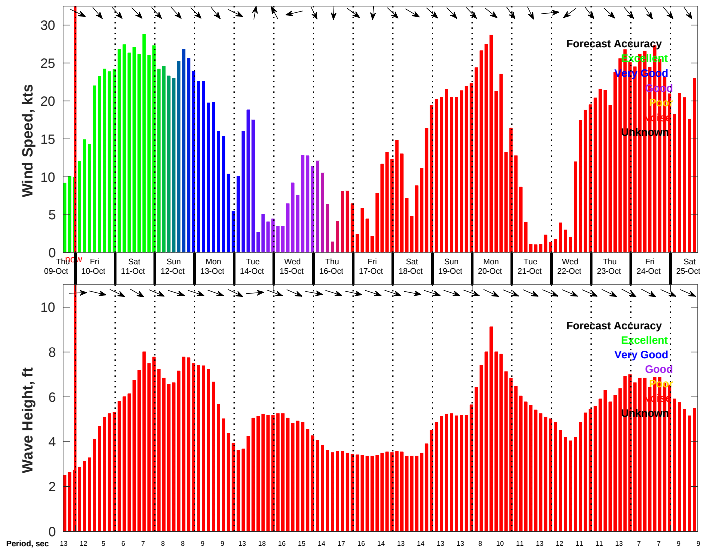
Wind & Wave Forecast for NDBC 46054 from 09-Oct-2025 16:00:00 to 25-Oct-2025 16:00:00
