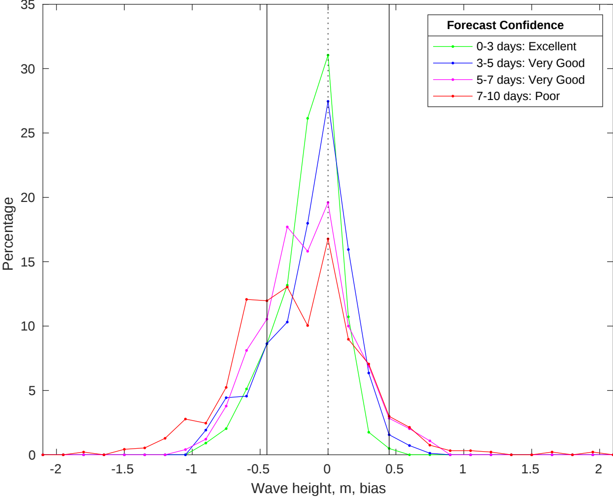
NDBC 46069 vs CMEMS Waves Bias Histogram: 10-Oct-2025
