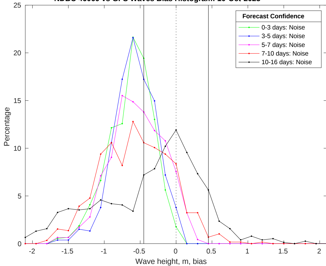
NDBC 46069 vs GFS Waves Bias Histogram: 10-Oct-2025
