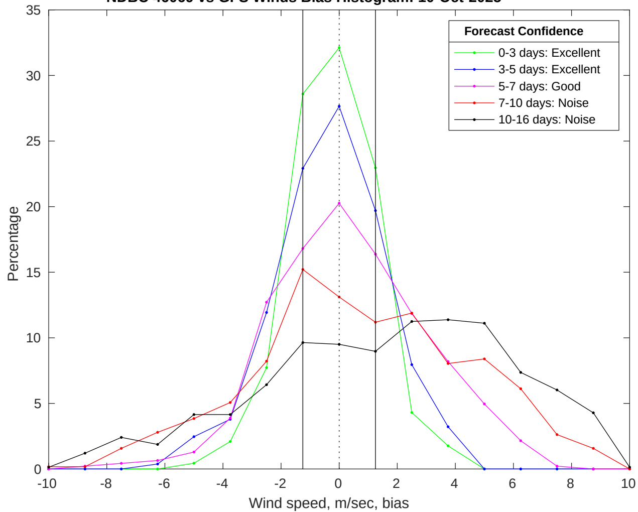
NDBC 46069 vs GFS Winds Bias Histogram: 10-Oct-2025
