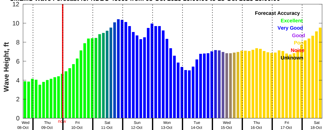
CMEMS Wave Forecast for NDBC 46069 from 08-Oct-2025 16:00:00 to 18-Oct-2025 16:00:00
