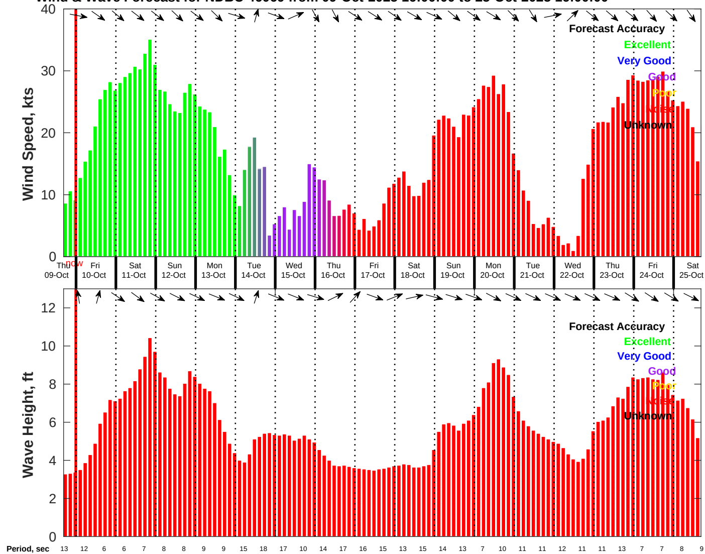
Wind & Wave Forecast for NDBC 46069 from 09-Oct-2025 16:00:00 to 25-Oct-2025 16:00:00
