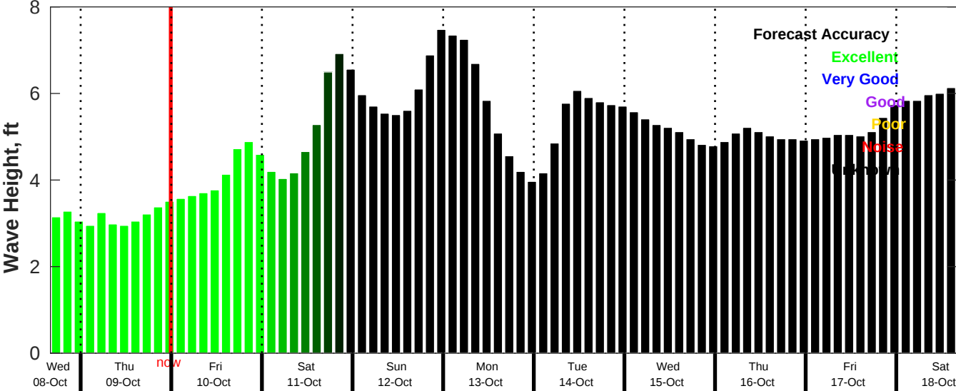
CMEMS Wave Forecast for NDBC 46215 from 08-Oct-2025 16:00:00 to 18-Oct-2025 16:00:00
