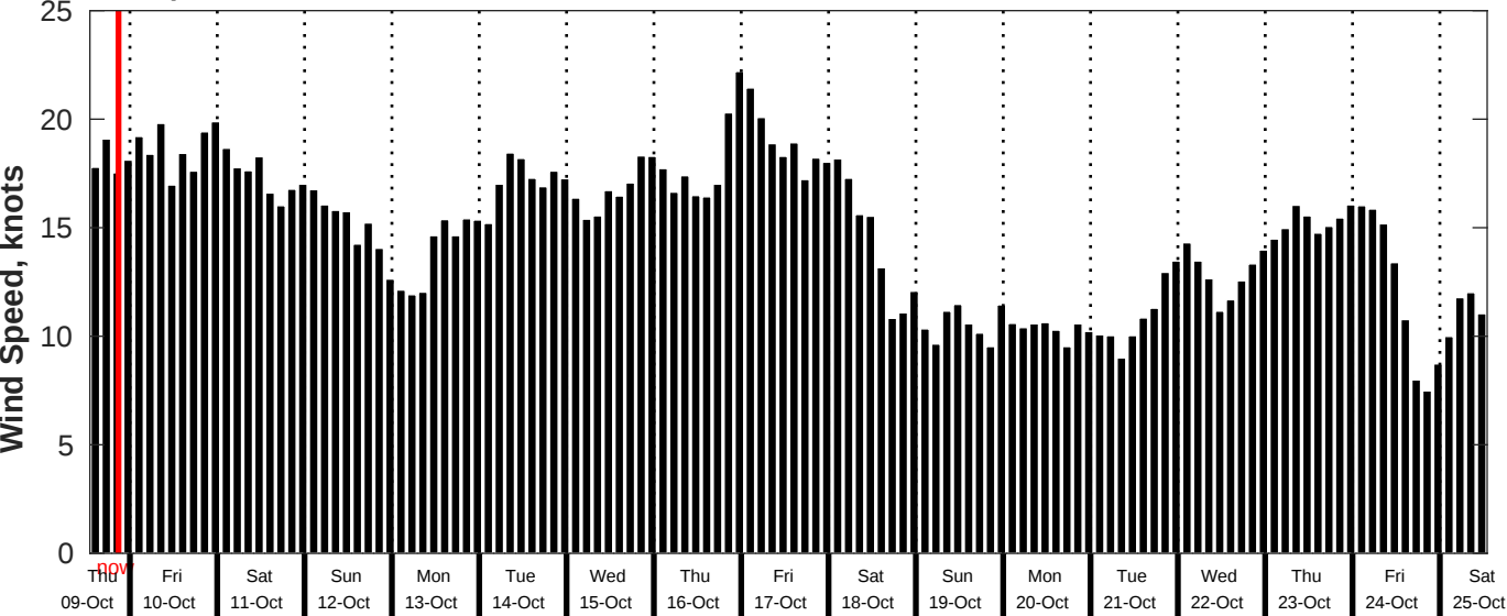
GFS Wind Speed Forecast for NDBC 51209 from 09-Oct-2025 13:00:00 to 25-Oct-2025 13:00:00
