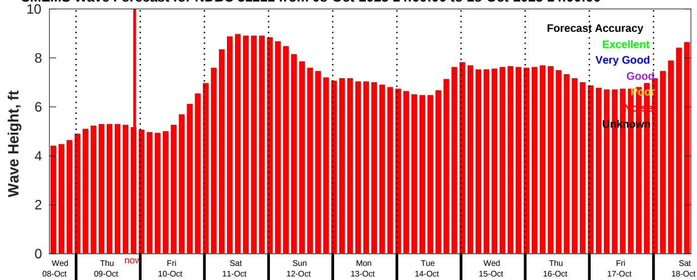
CMEMS Wave Forecast for NDBC 51211 from 08-Oct-2025 14:00:00 to 18-Oct-2025 14:00:00
