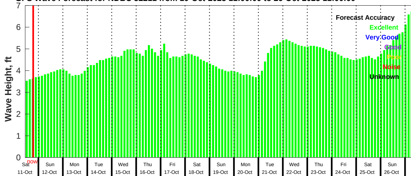
GFS Wave Forecast for NDBC 52211 from 10-Oct-2025 11:00:00 to 26-Oct-2025 11:00:00
