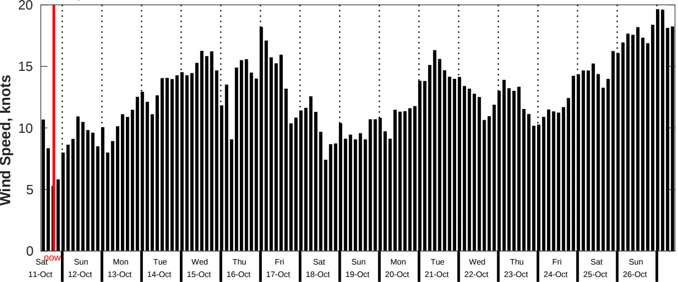
GFS Wind Speed Forecast for NDBC 52211 from 10-Oct-2025 11:00:00 to 26-Oct-2025 11:00:00
