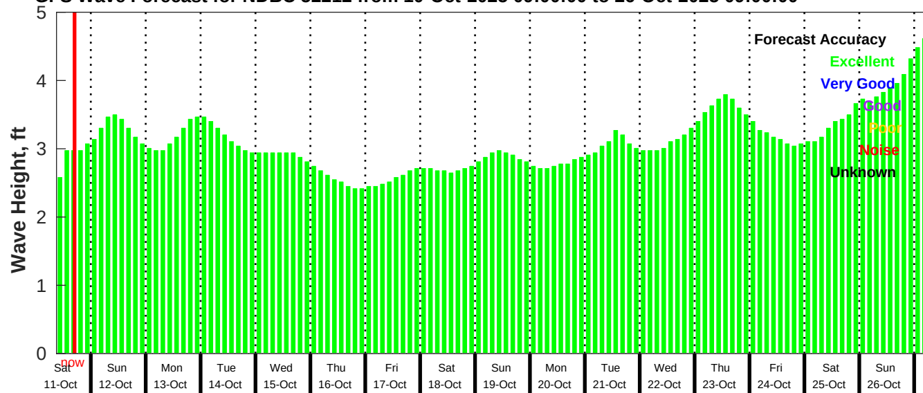
GFS Wave Forecast for NDBC 52212 from 10-Oct-2025 09:00:00 to 26-Oct-2025 09:00:00
