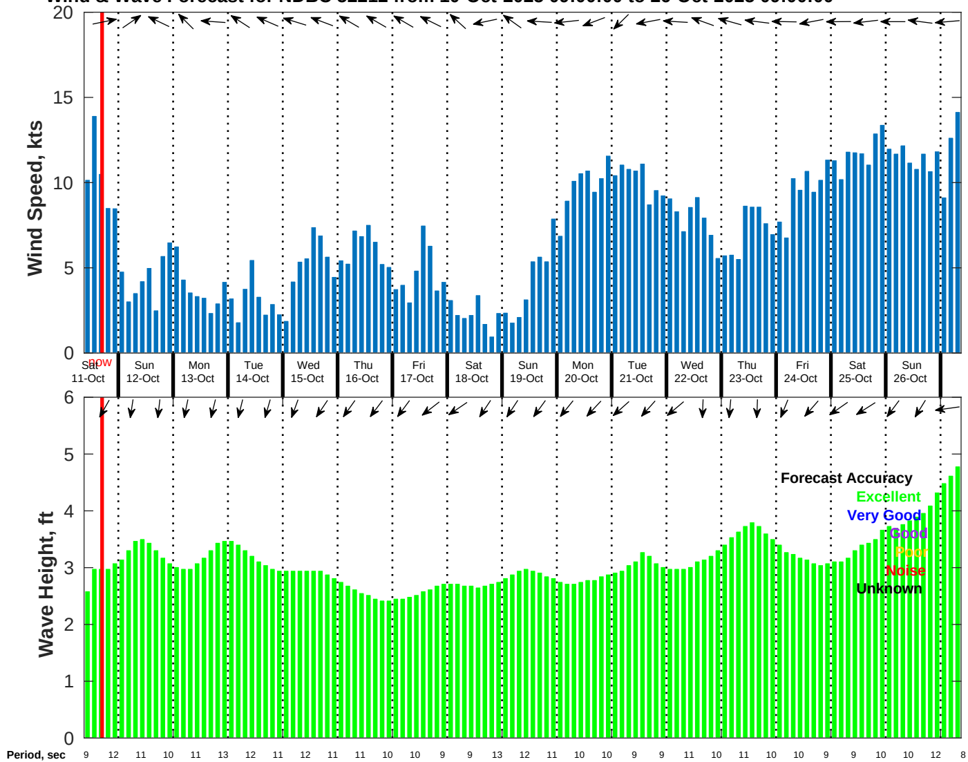
Wind & Wave Forecast for NDBC 52212 from 10-Oct-2025 09:00:00 to 26-Oct-2025 09:00:00
