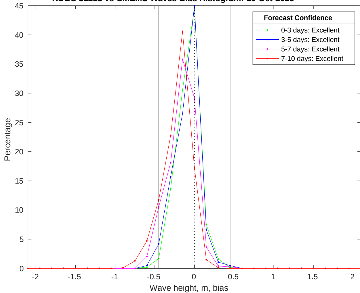
NDBC 52213 vs CMEMS Waves Bias Histogram: 10-Oct-2025
