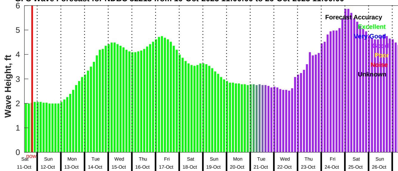
GFS Wave Forecast for NDBC 52213 from 10-Oct-2025 11:00:00 to 26-Oct-2025 11:00:00
