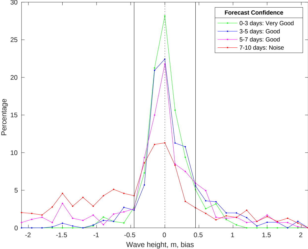
NDBC 41004 vs CMEMS Waves Bias Histogram: 11-Oct-2025
