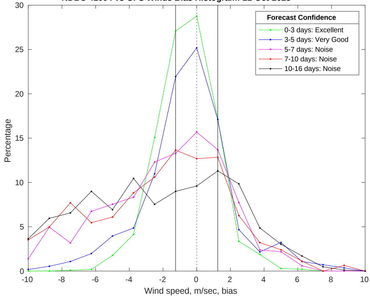
NDBC 41004 vs GFS Winds Bias Histogram: 11-Oct-2025
