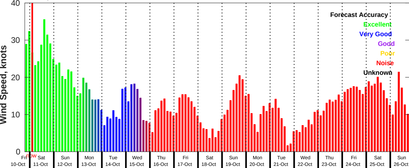
GFS Wind Speed Forecast for NDBC 41004 from 10-Oct-2025 19:00:00 to 26-Oct-2025 19:00:00
