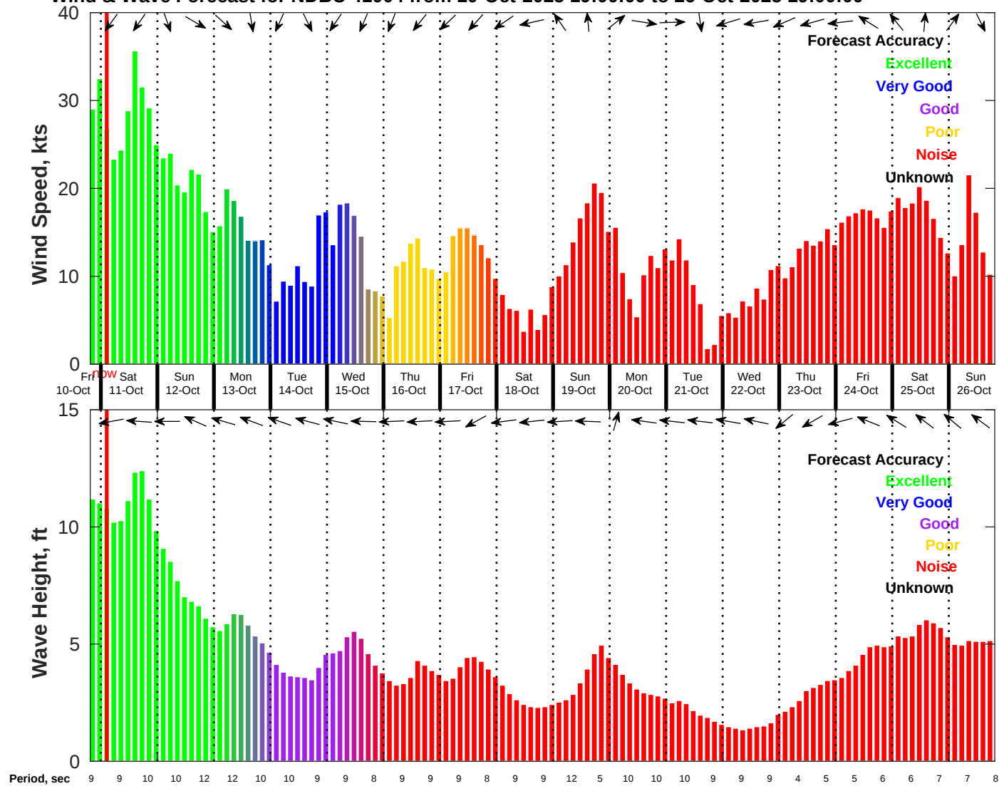
Wind & Wave Forecast for NDBC 41004 from 10-Oct-2025 19:00:00 to 26-Oct-2025 19:00:00
