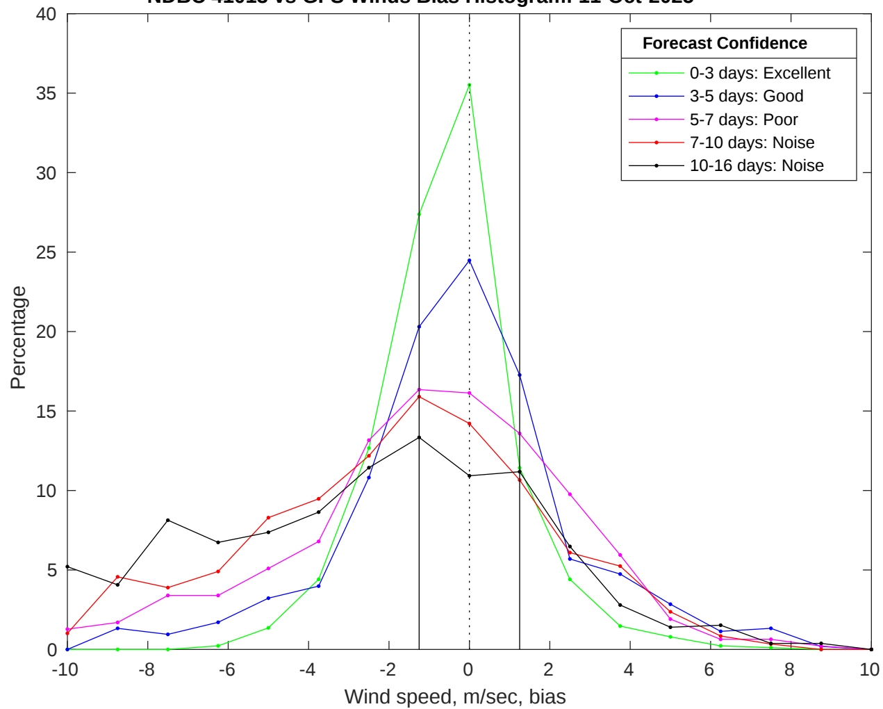
NDBC 41013 vs GFS Winds Bias Histogram: 11-Oct-2025
