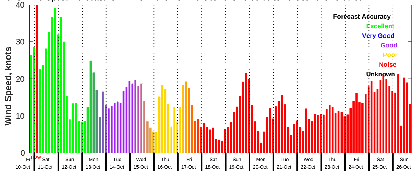
GFS Wind Speed Forecast for NDBC 41013 from 10-Oct-2025 19:00:00 to 26-Oct-2025 19:00:00
