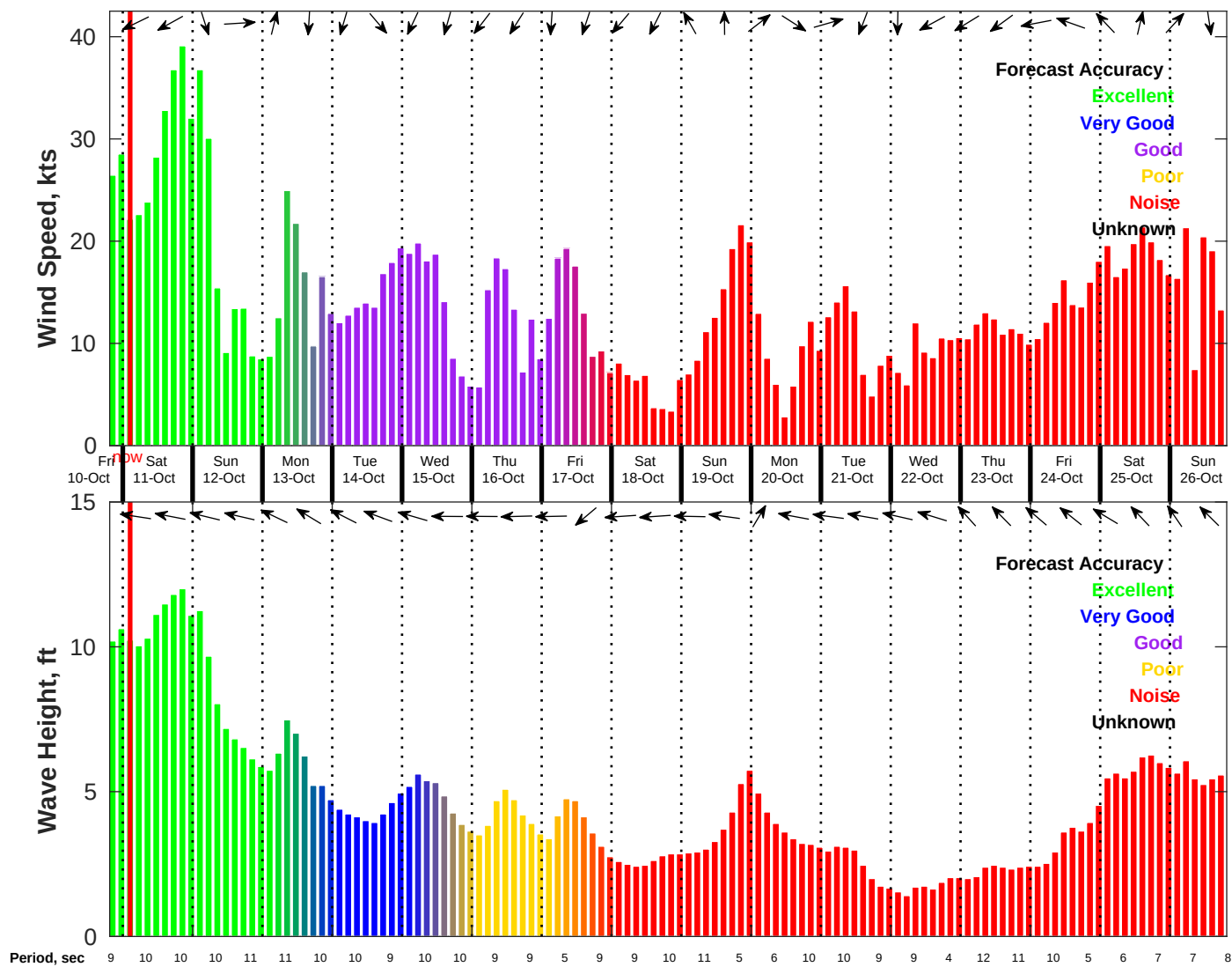
Wind & Wave Forecast for NDBC 41013 from 10-Oct-2025 19:00:00 to 26-Oct-2025 19:00:00
