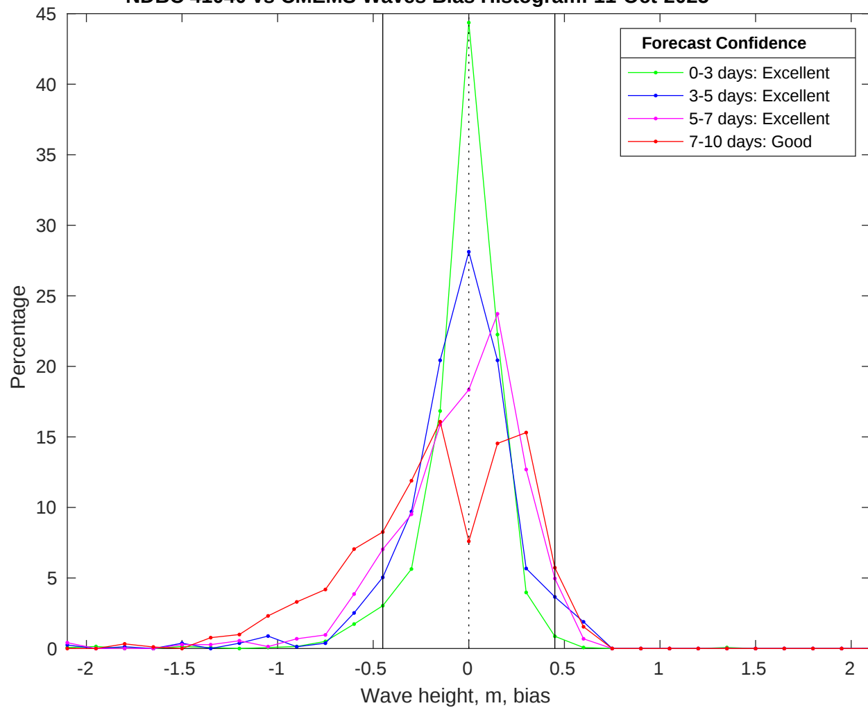
NDBC 41040 vs CMEMS Waves Bias Histogram: 11-Oct-2025
