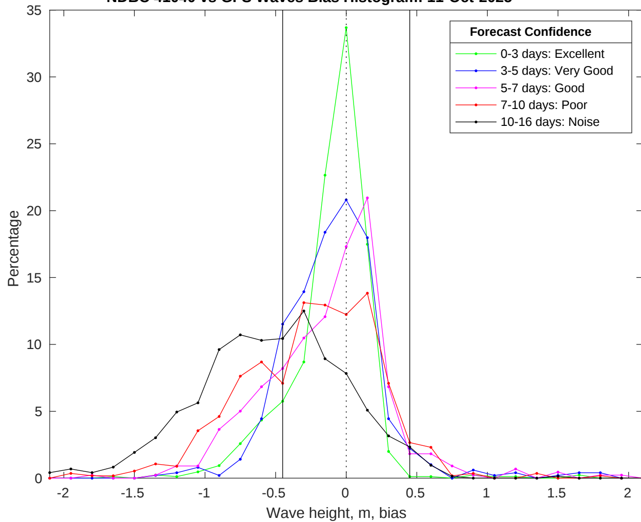
NDBC 41040 vs GFS Waves Bias Histogram: 11-Oct-2025
