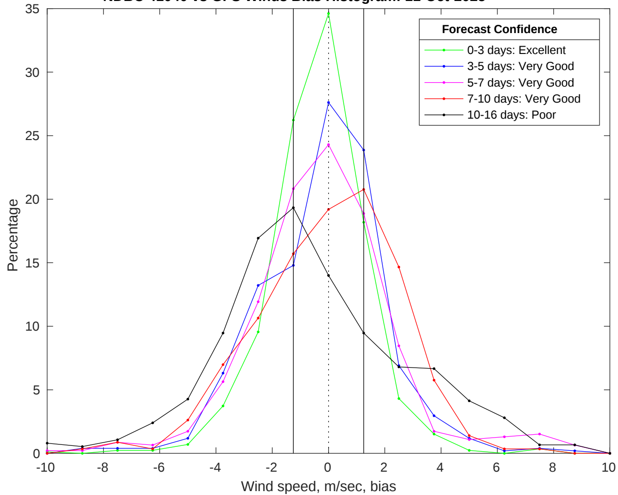
NDBC 41040 vs GFS Winds Bias Histogram: 11-Oct-2025
